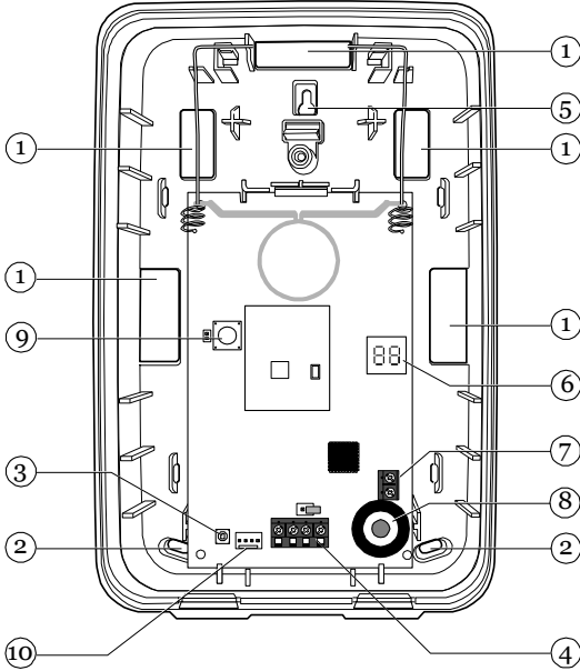
Figure 10 Extension Radio
