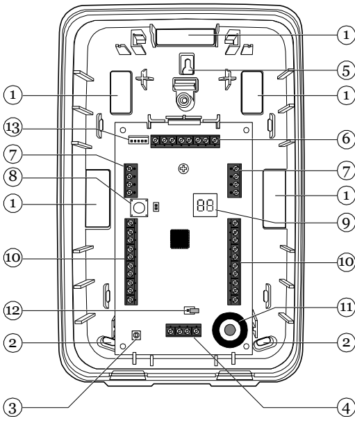
Figure 9 Extension Filaire
