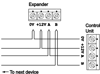
Figure 21 Câblage Extension
